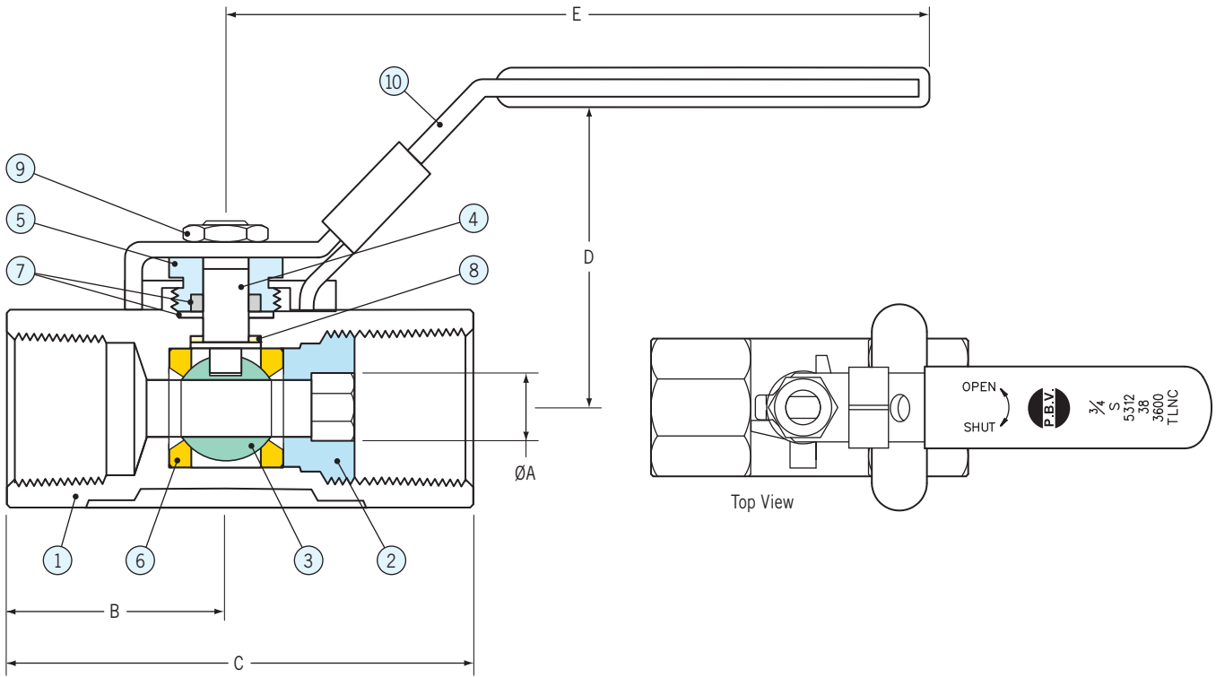
Dimensional Data (in.) Cv & Wt. (lbs.) • 1/4" - 2"
