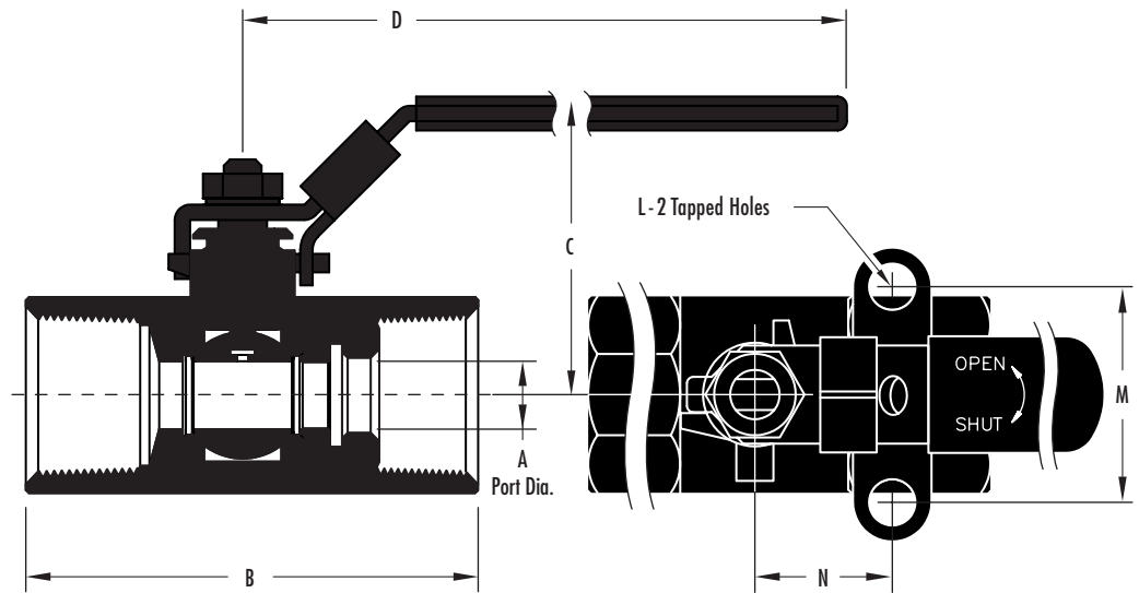
5312 Dimensional Data (in.), C v Data and Weight (lbs.) ■ 1/4"-2"
